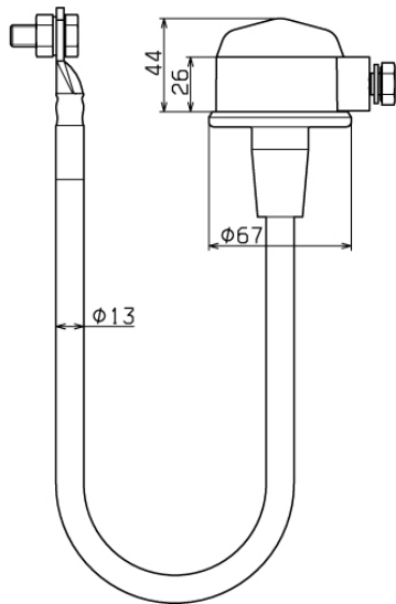
Dimension Drawing EXFS
