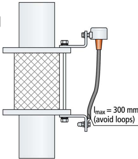
Installation of EXFS
